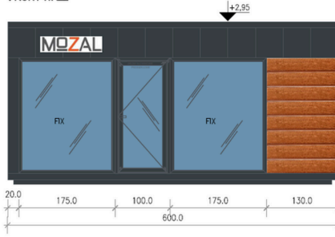
FRONT WALL
