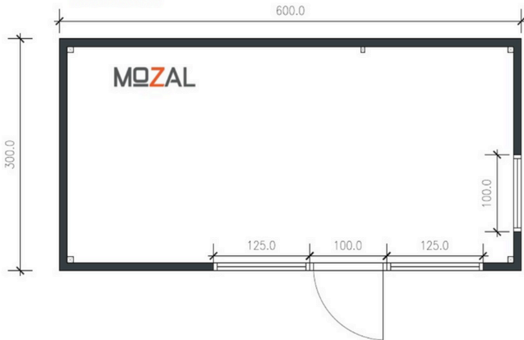
FLOOR PLAN
